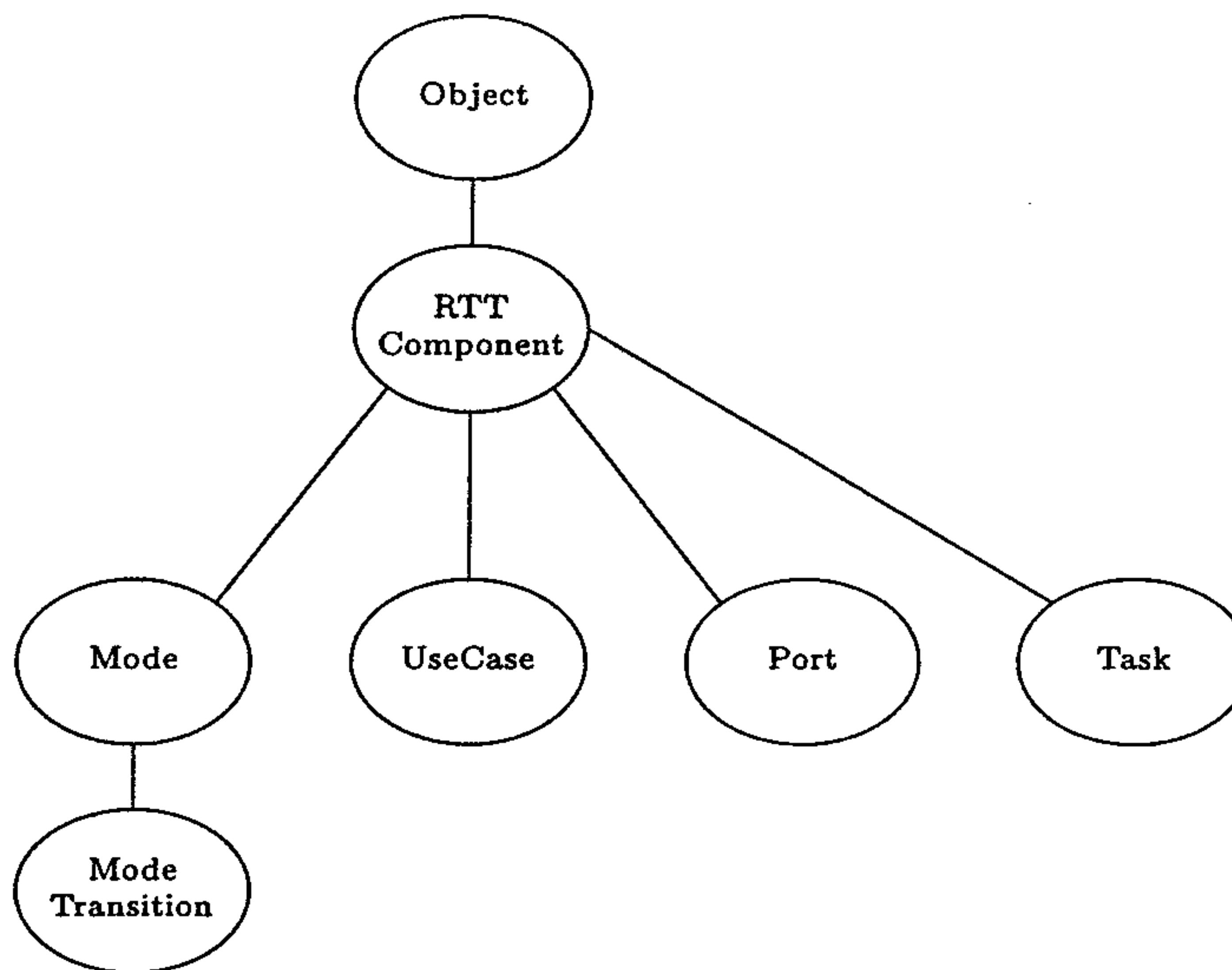
FIG. 7. Class hierarchy.
